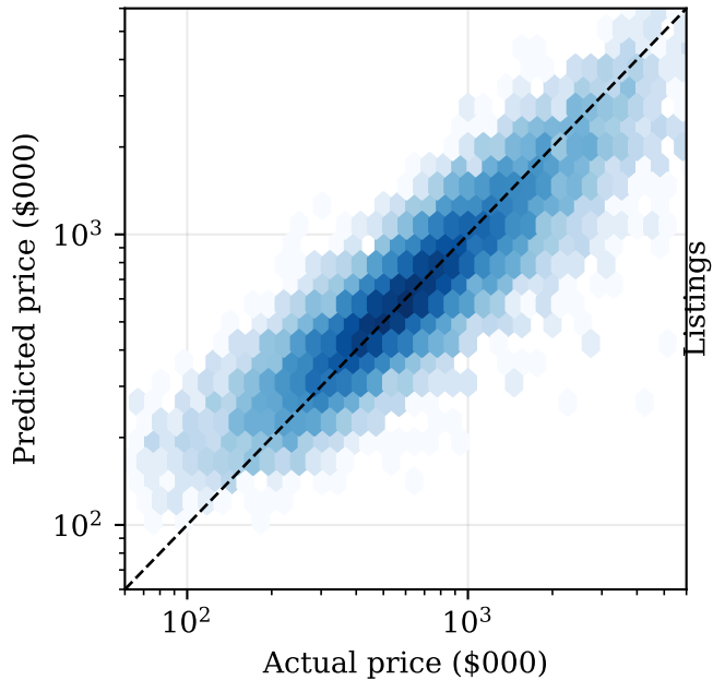
Calibration (blend, R^2=0.779 )
