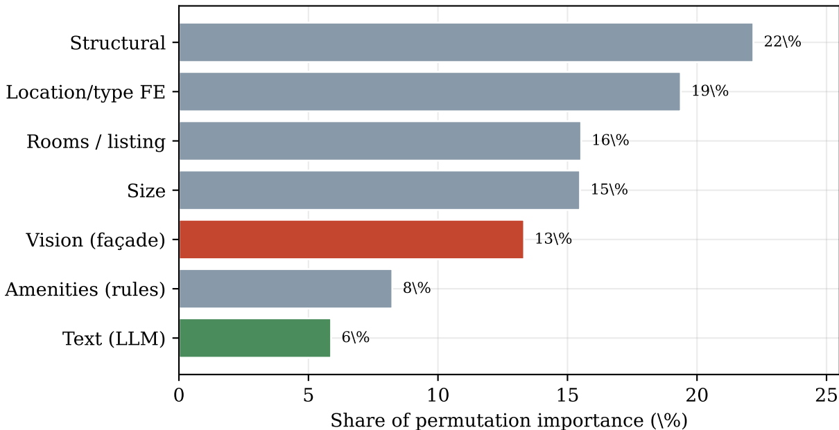
Feature-block importance (gradient boosting, v5)
