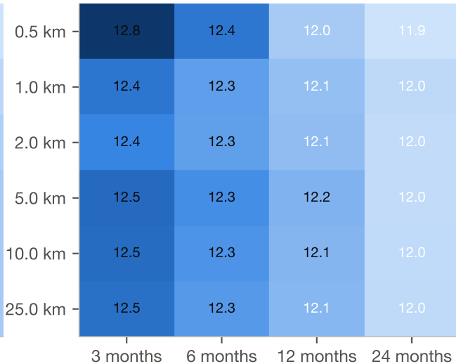
hedonic grid — MdAPE at the best k
