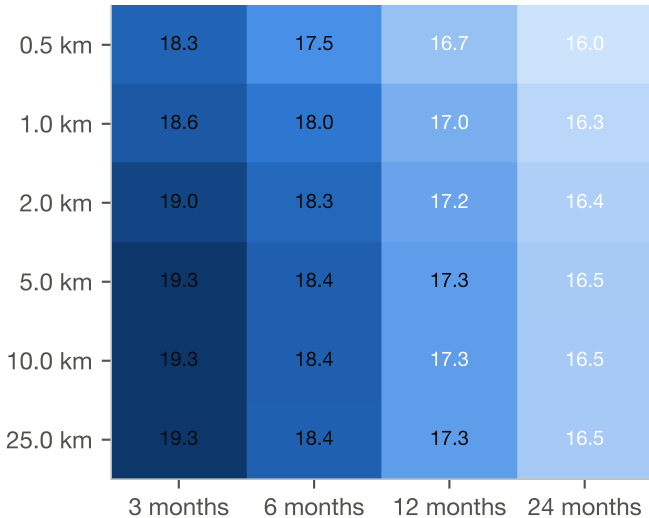
time adjustment only — MdAPE at the best k
