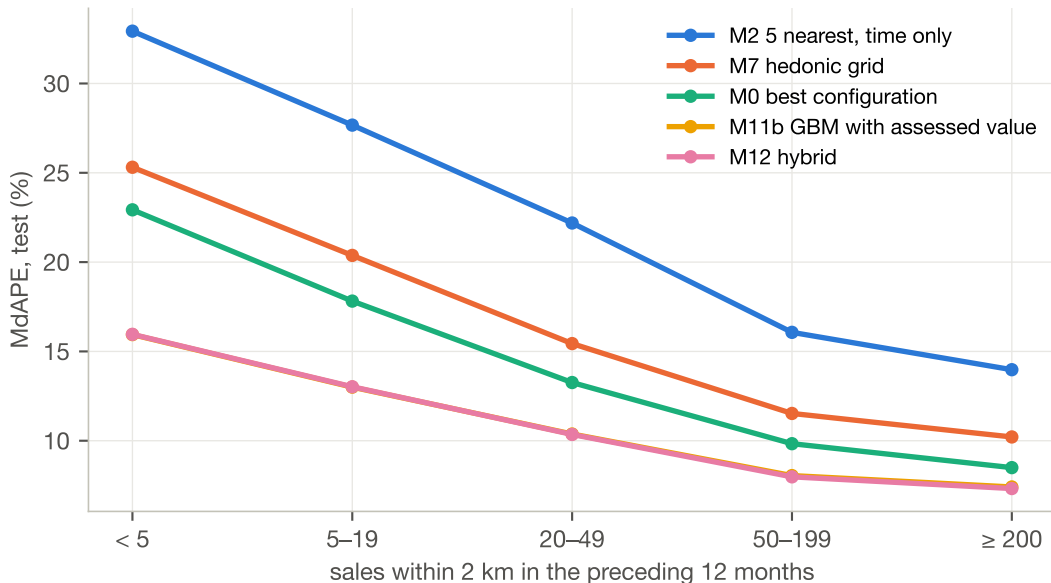
Accuracy by submarket liquidity
