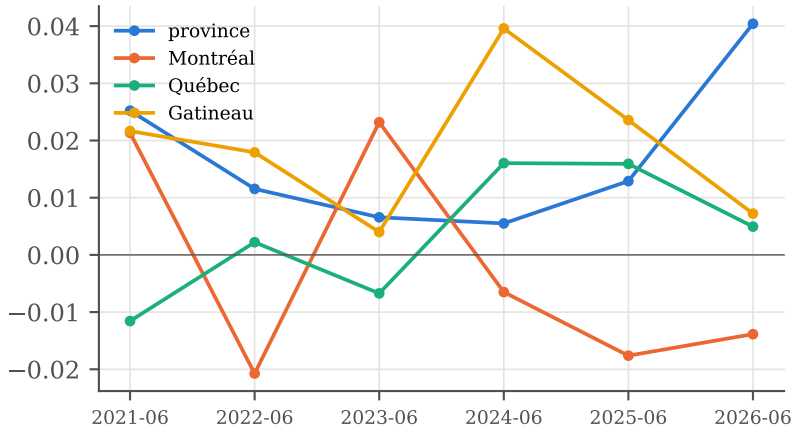
Moran's I of stage-1 residuals (10-N)
