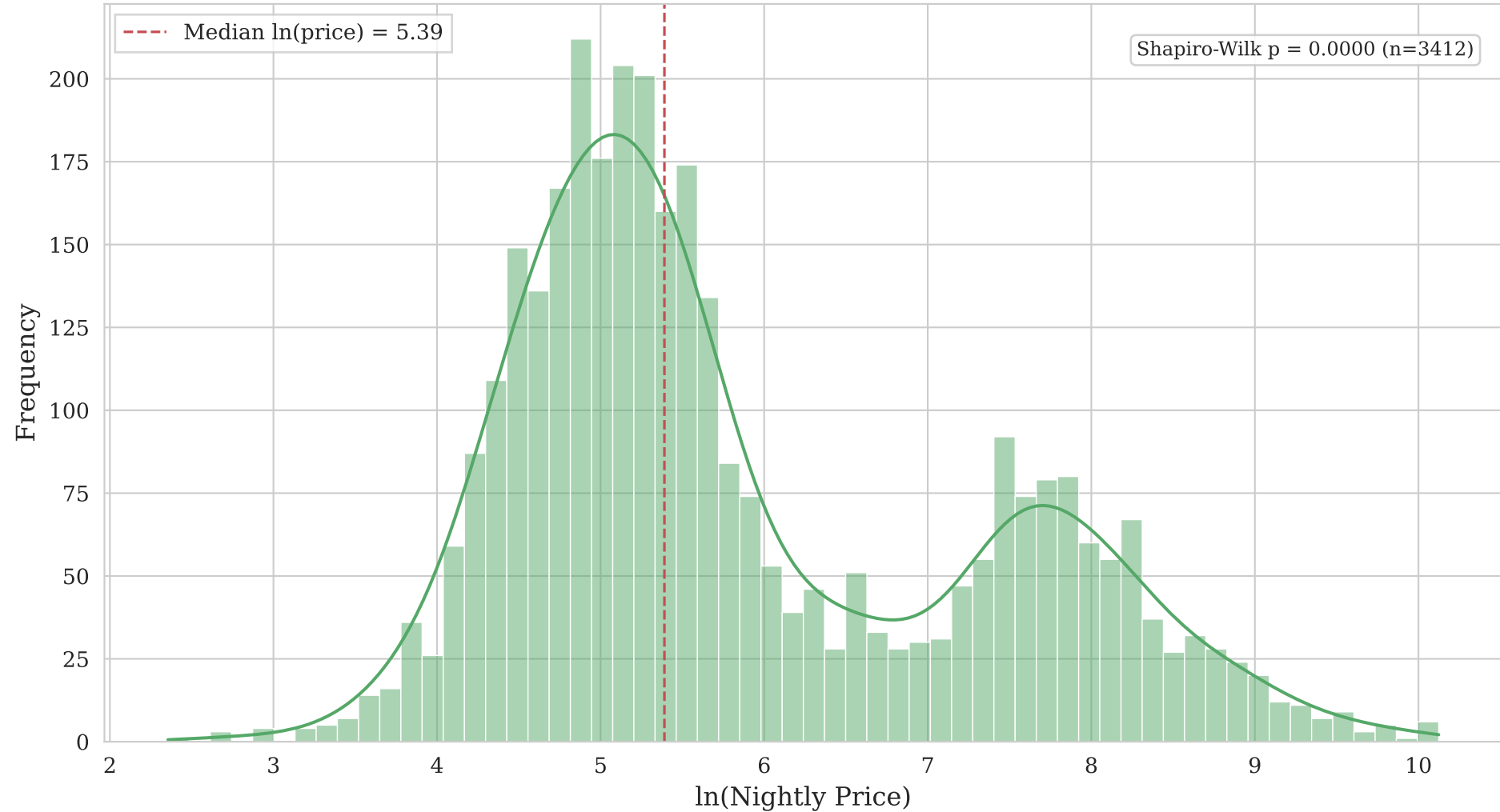
Distribution of Log-Transformed Prices (Semi-log hedonic model dependent variable)
