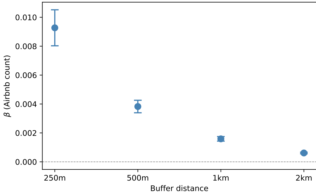
Airbnb Count Coefficient by Buffer Distance (95% CI)
