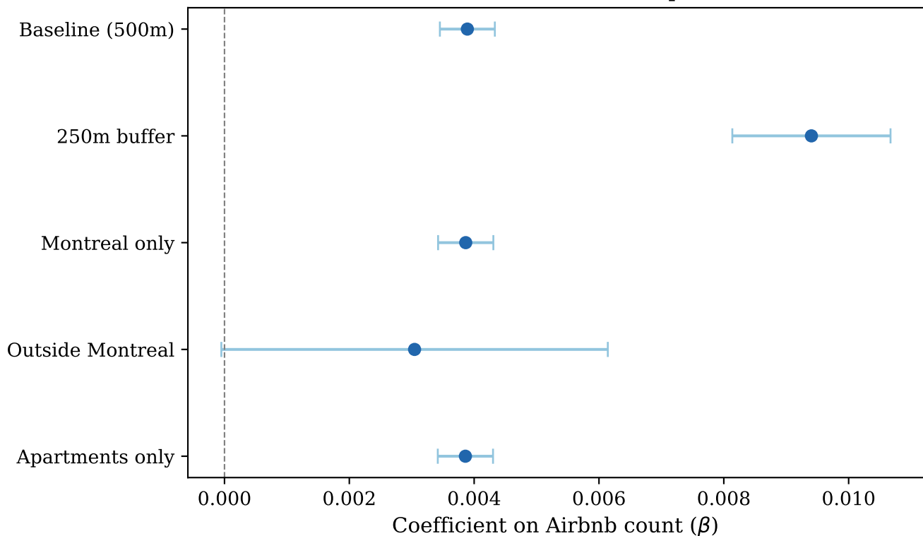
Coefficient Robustness Across Specifications
