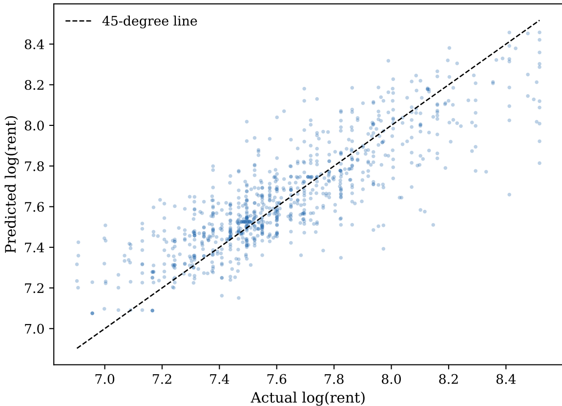
Predicted vs Actual — Random Forest (test R^2=0.7079 )
