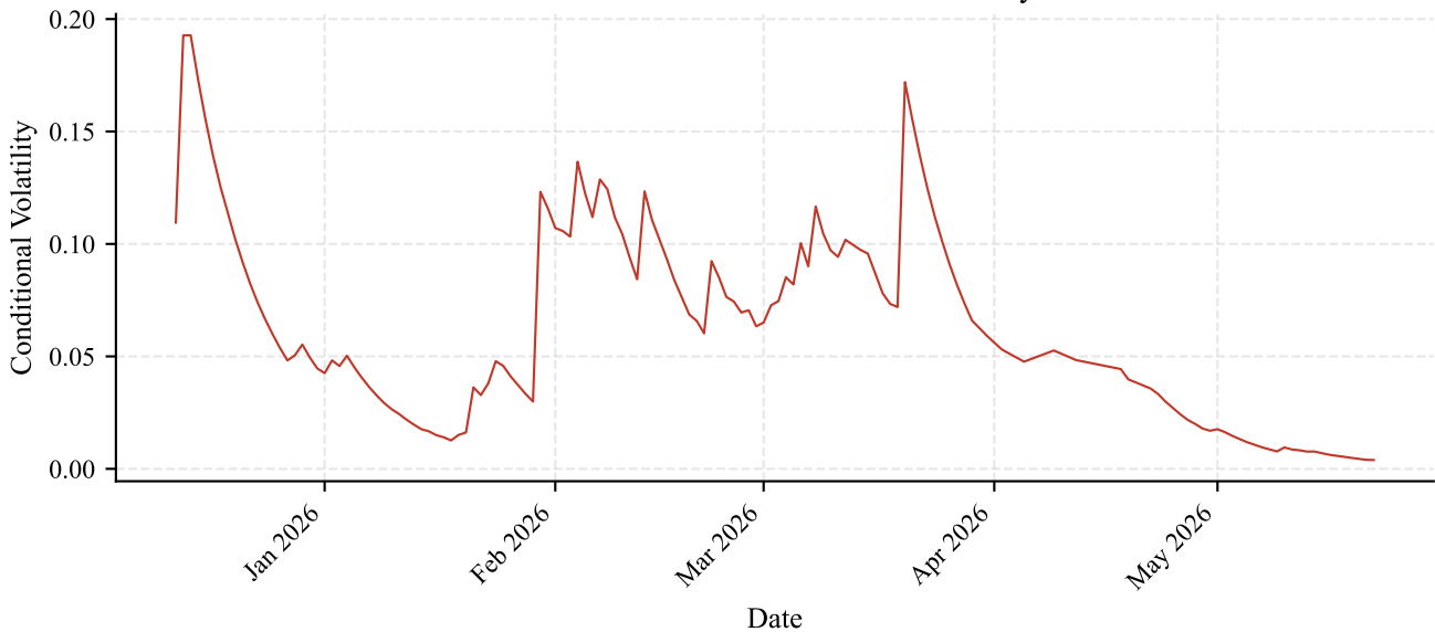
Panel B: GARCH Conditional Volatility
